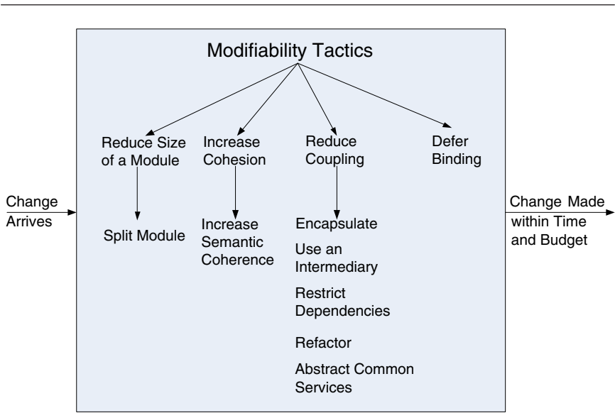
FIGURE 7.3 Modifiability tactics
